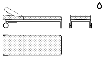
Lounger with castors L 205 P 76 H 47 cm W 80 6 / 8 " D 29 7 / 8 " H 18 4 / 8 "
