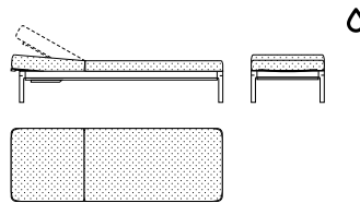
Lounger L 205 P 70 H 47 cm W 80 6 / 8 " D 27 1 / 4 " H 18 4 / 8 "
